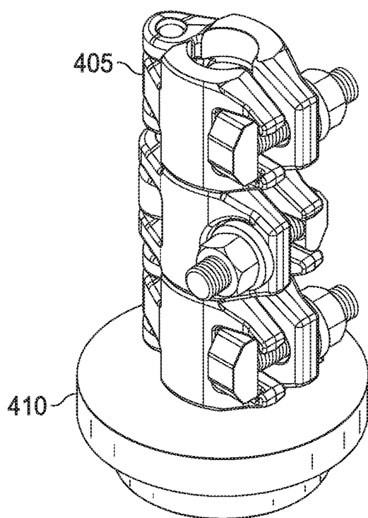
FIG. 4A (PRIOR ART)
